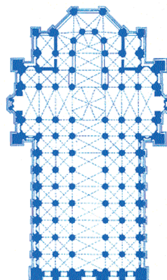
Floor-plan of Duomo of Milan.
